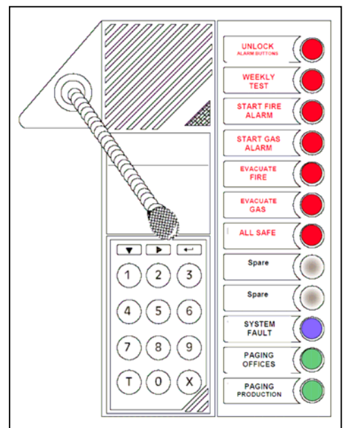
Model EE380/K12 Supervised microphone station 12 buttons. (Model EE380/K24 and K48 will have 24 or 48 buttons)
